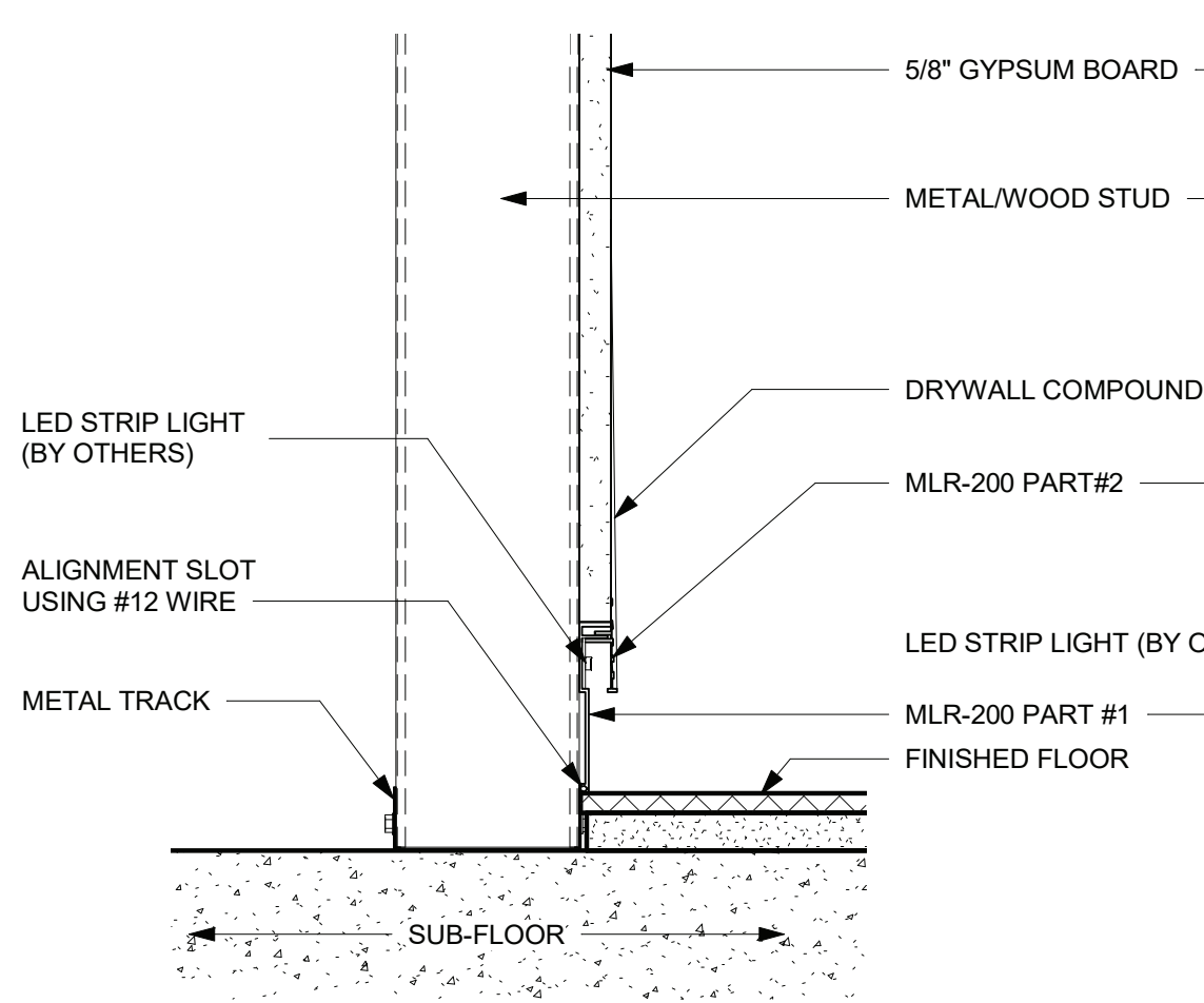
1 Section 1 3" = 1'-0"
